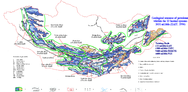
Geological map of Mongoli
